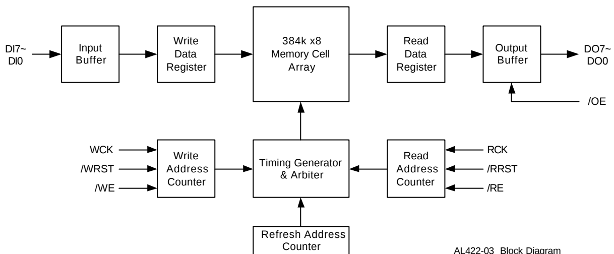
AL422-03 Block Diagram
